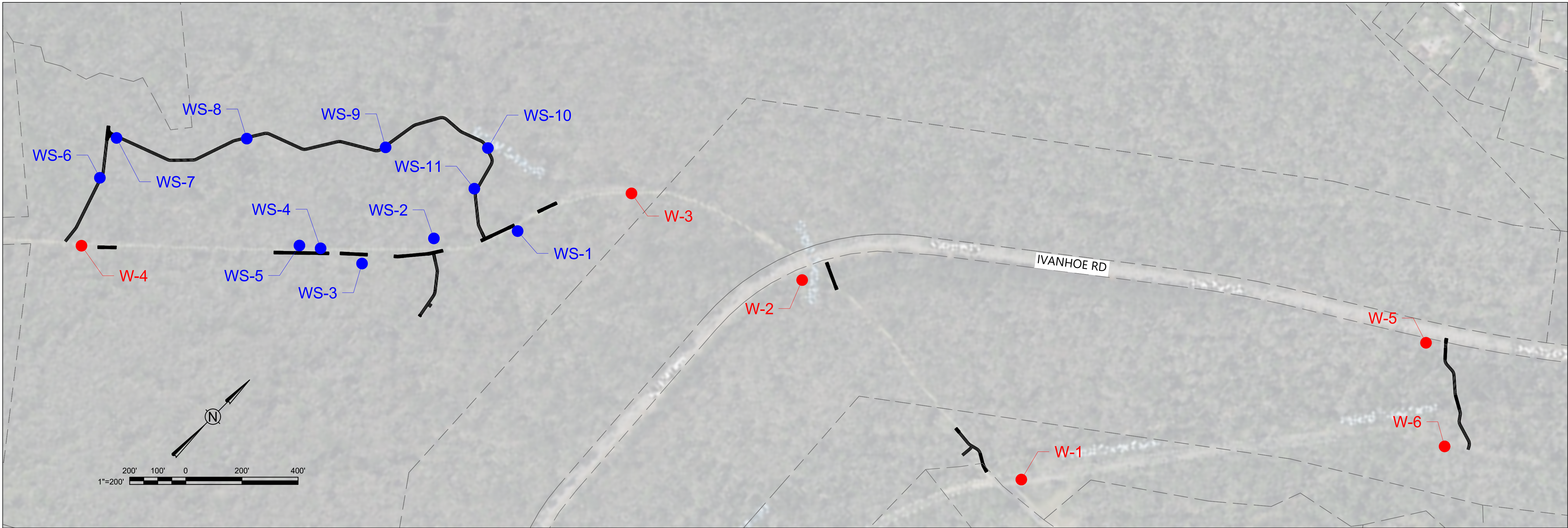
BORING LOCATION PLAN AERIAL IMAGERY COURTESY OF MICROSOFT CORPORATION, 2024 SCALE: 1"=200'
